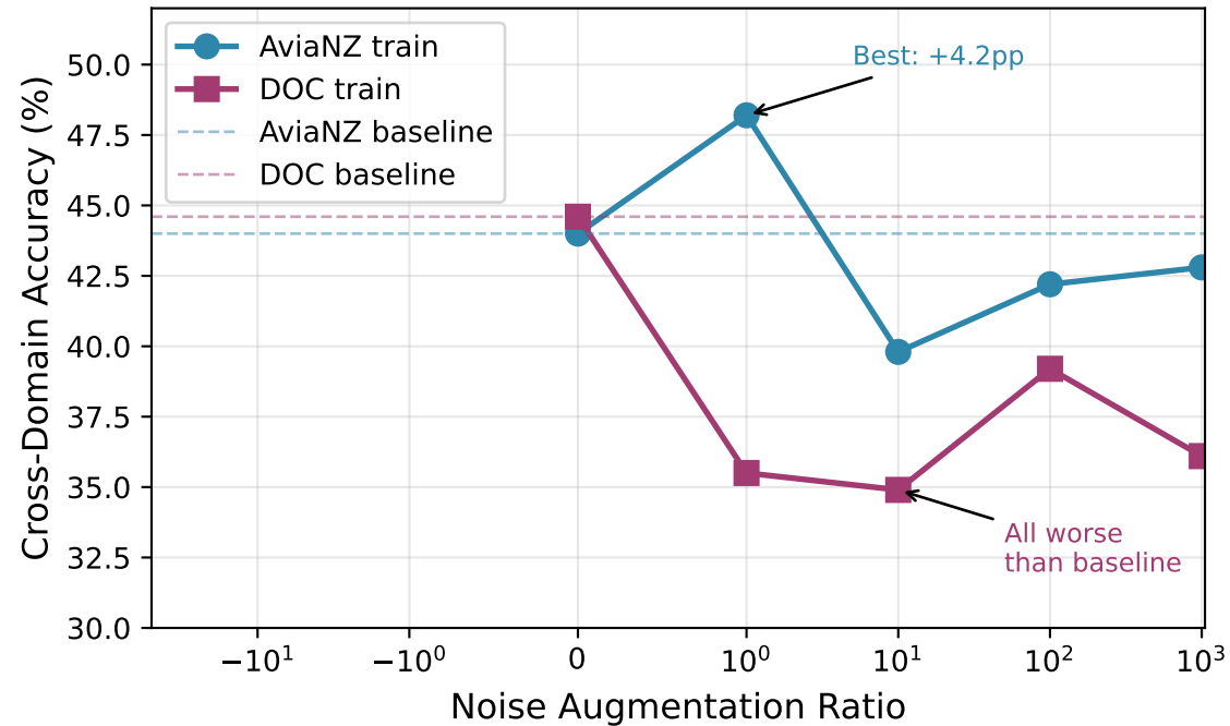
Cross-Domain Performance vs Noise Augmentation
