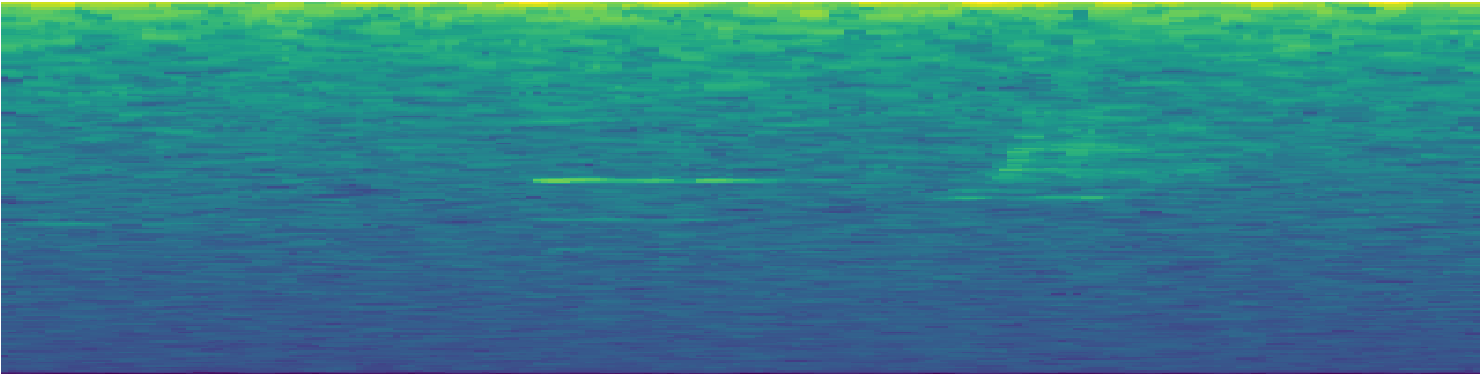
(c) Log+normalize
