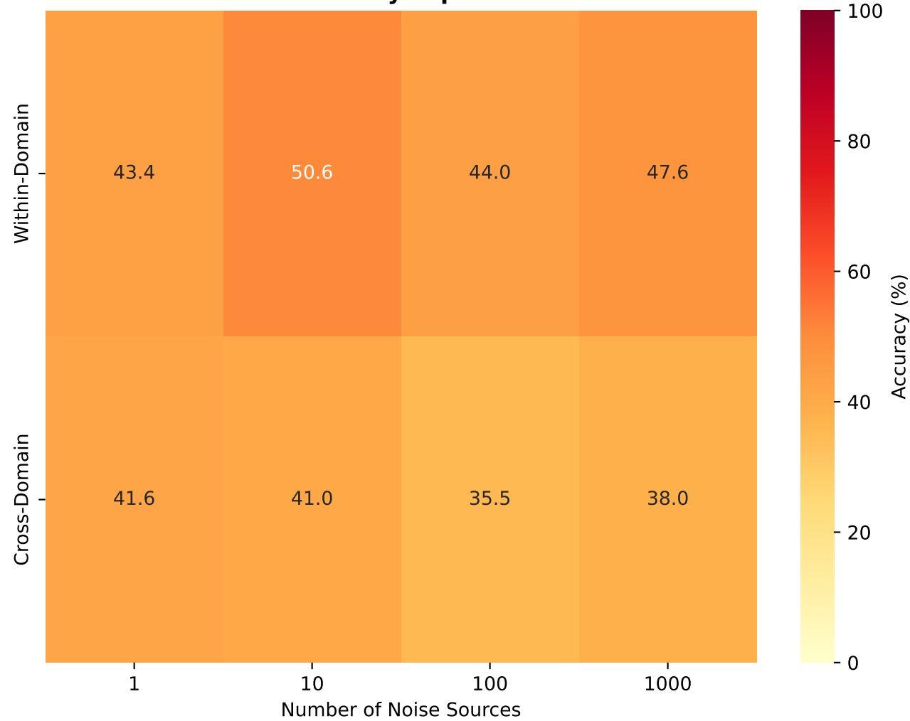
AviaNZ Training Noise Variety Experiments
