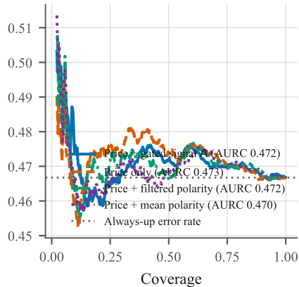
H = 5 sessions
