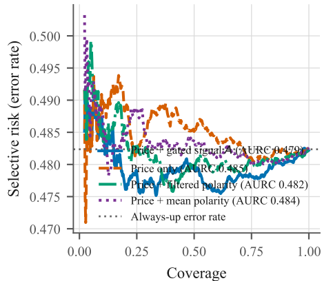
H = 1 session
