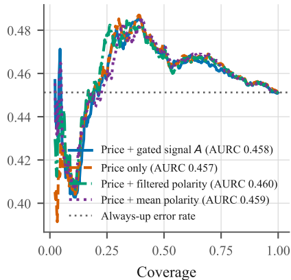
H = 21 sessions
