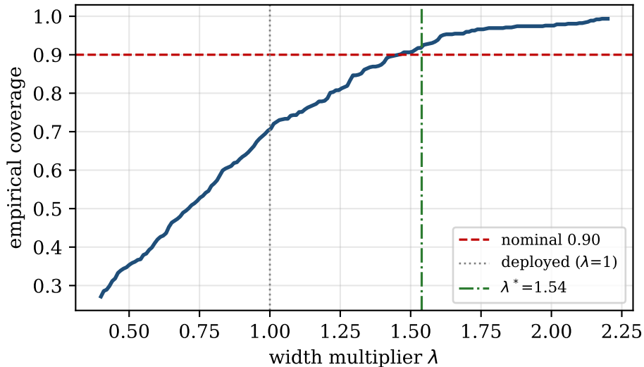
Coverage vs. interval-width multiplier
