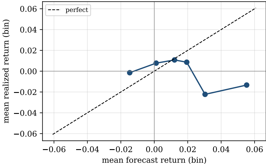
Forecast reliability curve (point forecast)
