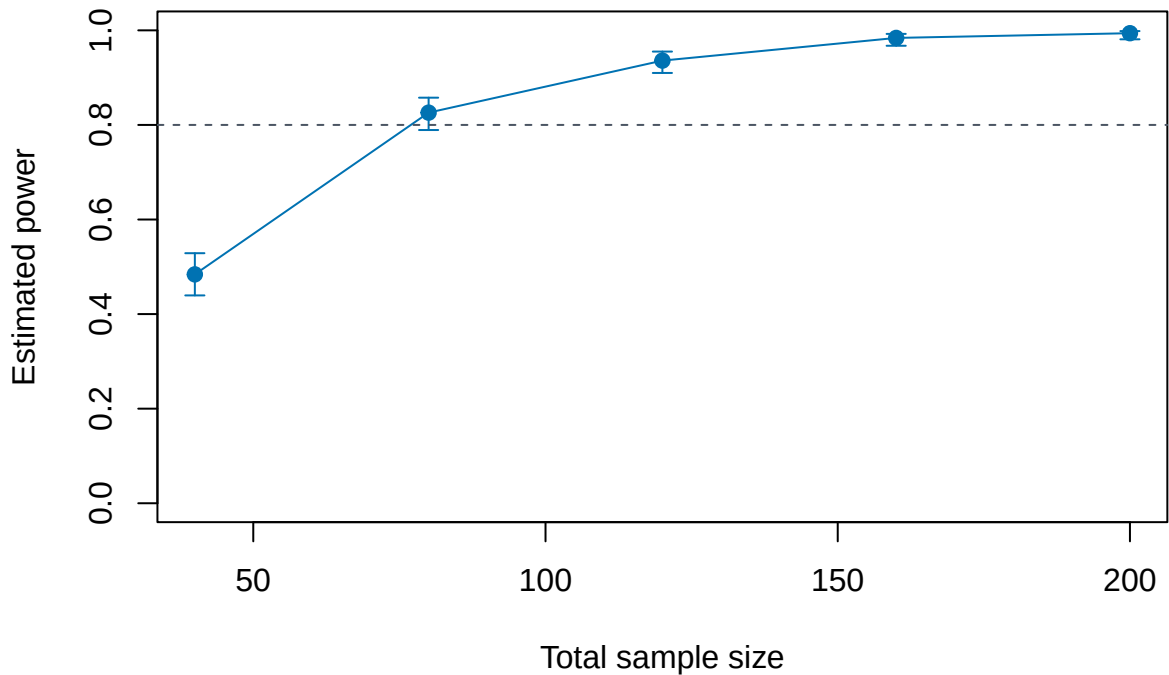
Figure 2: Power by sample size
