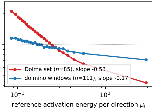
OLMo-3 7B, layers 23-25, input side
