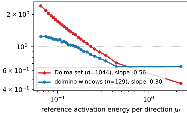
OLMo-2 7B, layers 23-25, input side
