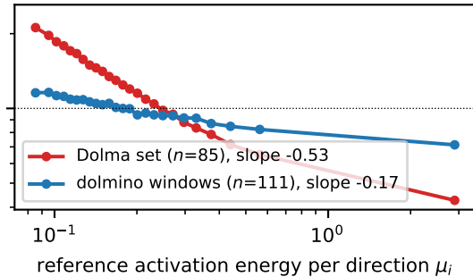
OLMo-3 7B, layers 23-25, input side
