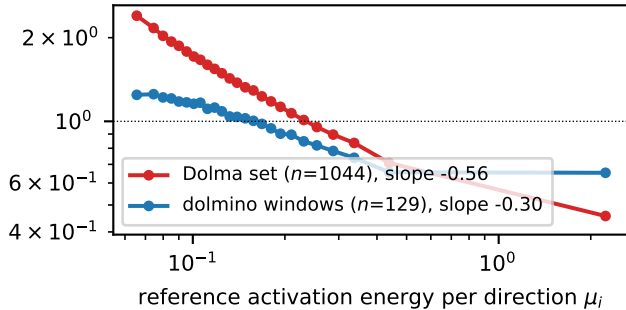
OLMo-2 7B, layers 23-25, input side
