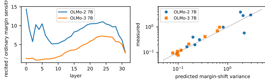
Figure 4: The layer map and its test. Left: ratio of recited to ordinary margin sensitivity per layer (Section 4.2) in both 7B models. Right: predicted against measured margin-shift variance under isotropic noise of per-matrix norm 60 on five three-layer bands, recited and ordinary tokens, no free parameter.
