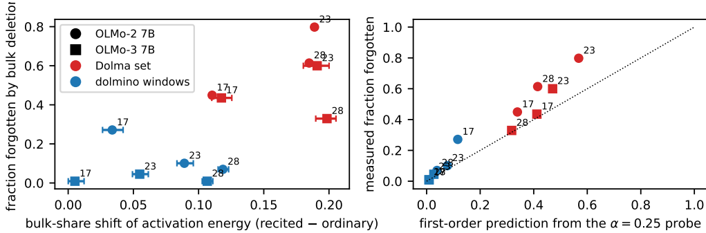
Figure 2: Deletability. Left: fraction of a population’s recitation removed by deleting the bulk block of a three-layer band, against the shift of the population’s activation bulk share relative to ordinary text (bootstrap 95% intervals over items), for two models, two populations and three bands (labels give the first layer of the band). Right: the same fraction against the first-order prediction from a quarter-deletion probe (Proposition 2).
