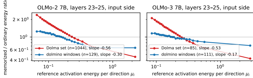
Figure 1: Whitening profiles. Ratio of the memorized population’s mean activation energy per direction to ordinary text’s, against the reference energy of the direction (binned over the input eigenbasis of the first matrix of the band, 25 bins), for the Dolma set and the recited dolmino windows in OLMo-2 7B and OLMo-3 7B. Slopes are least-squares exponents over all directions. The pretraining-era Dolma populations are whitened at -0.55 to -0.67 ; the late boilerplate at -0.2 to -0.33 .
