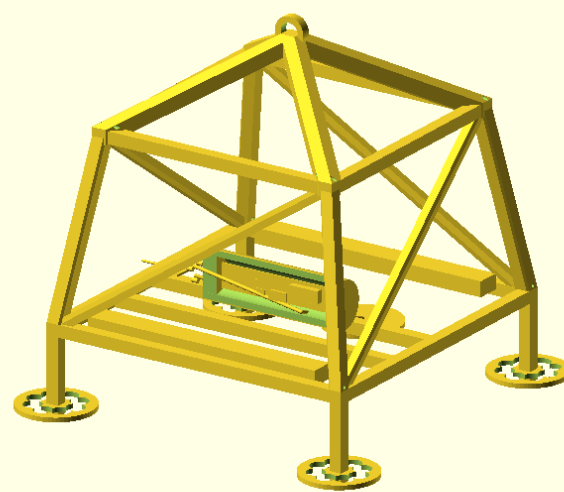
Payload carrier and lander
