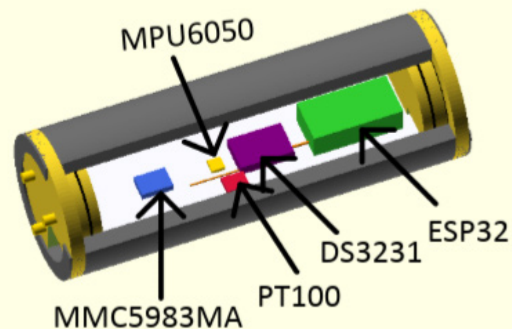
Payload carrier and lander
