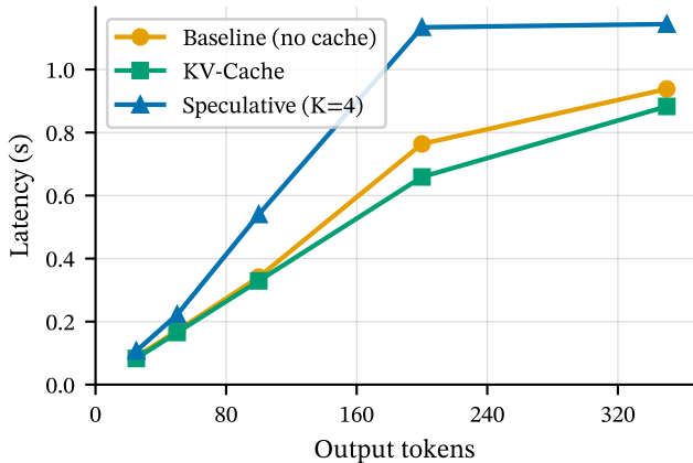
Inference Latency vs Sequence Length
