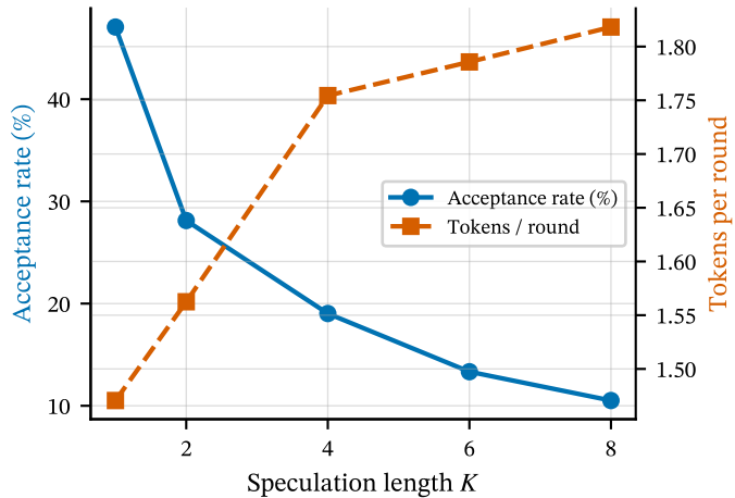
Draft Acceptance Analysis
