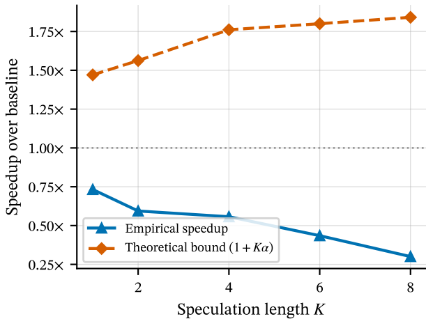
Empirical vs Theoretical Speedup
