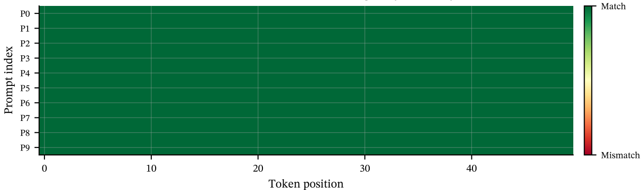
Output Equivalence: Baseline \equiv KV-Cache (greedy, token-by-token)
