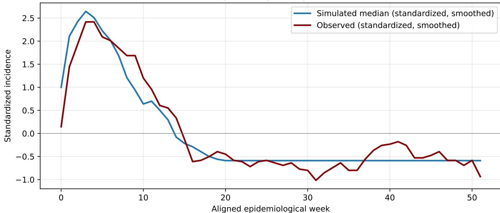
Temporal shape comparison
