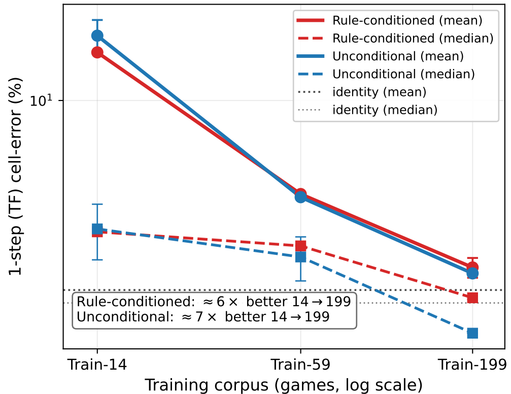
Out-of-distribution (Heldout-26)
