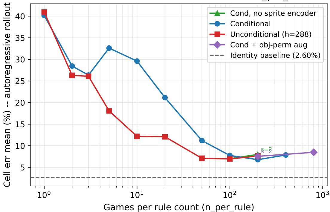
OOD Heldout-26: AR rollout mean error vs n_per_rule
