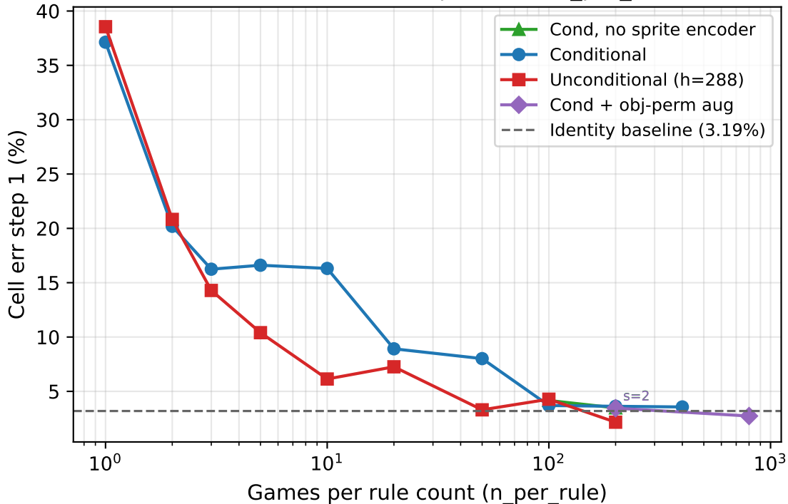
OOD Heldout-26: 1-step error vs n_per_rule
