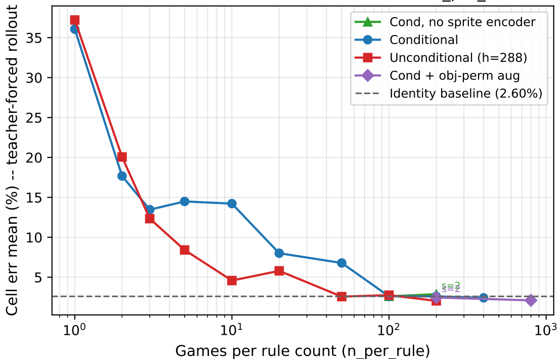
OOD Heldout-26: TF rollout mean error vs n_per_rule
