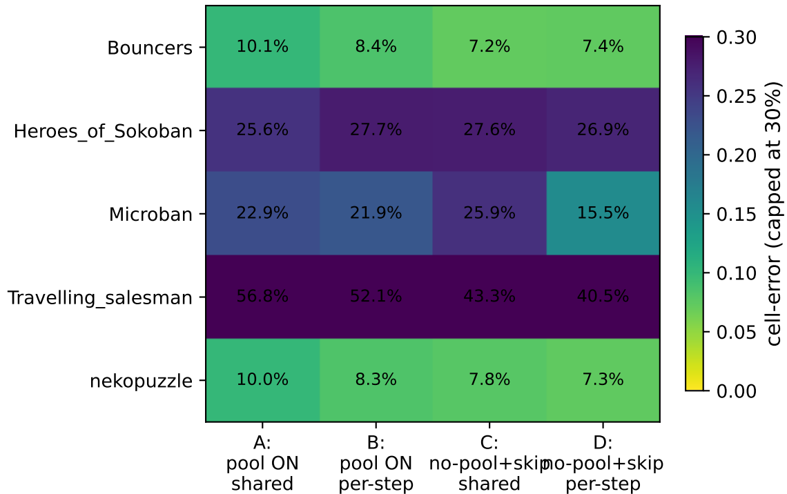
BFS cell-error — held-out levels (L1+ mean)
