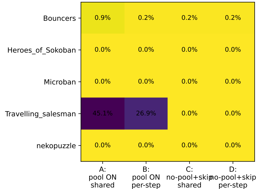
BFS cell-error — training level (L0)
