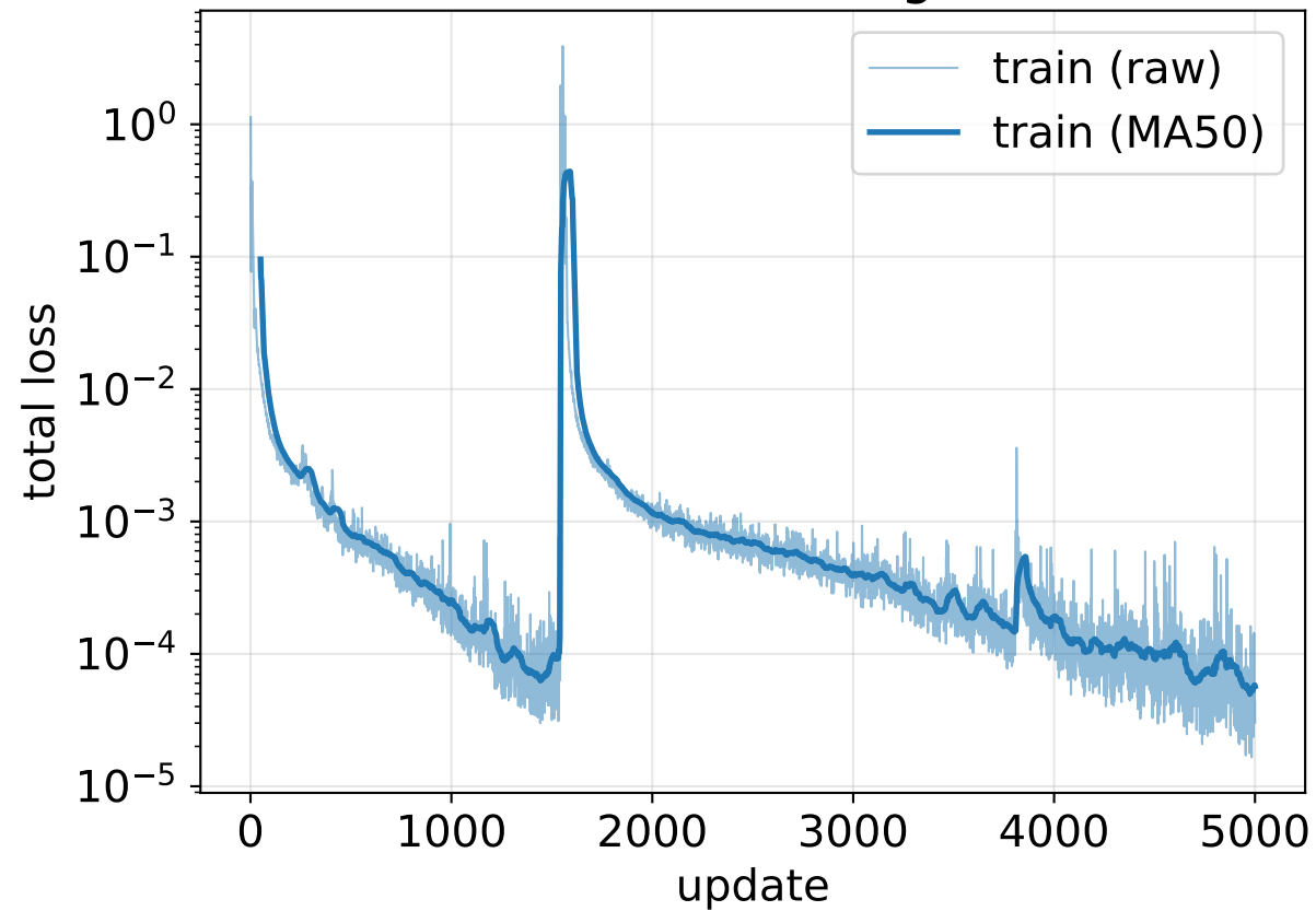
Mario WM training loss
