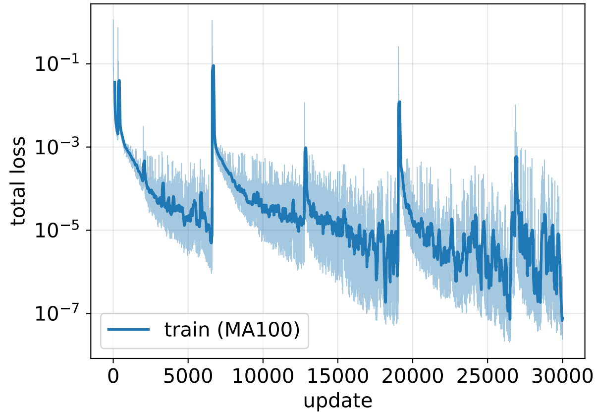
Mario WM loss (30k, full-batch, lr 2e-4)
