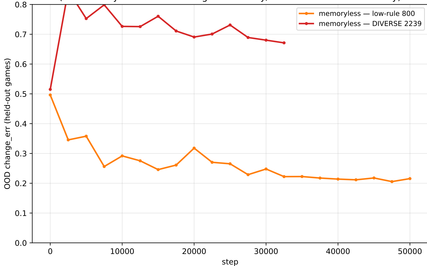
Memoryless OOD: low-rule corpus is learnable, diverse corpus is not (diverse stays \sim 0.68 \rightarrow needs game identity/context = room for memory)
