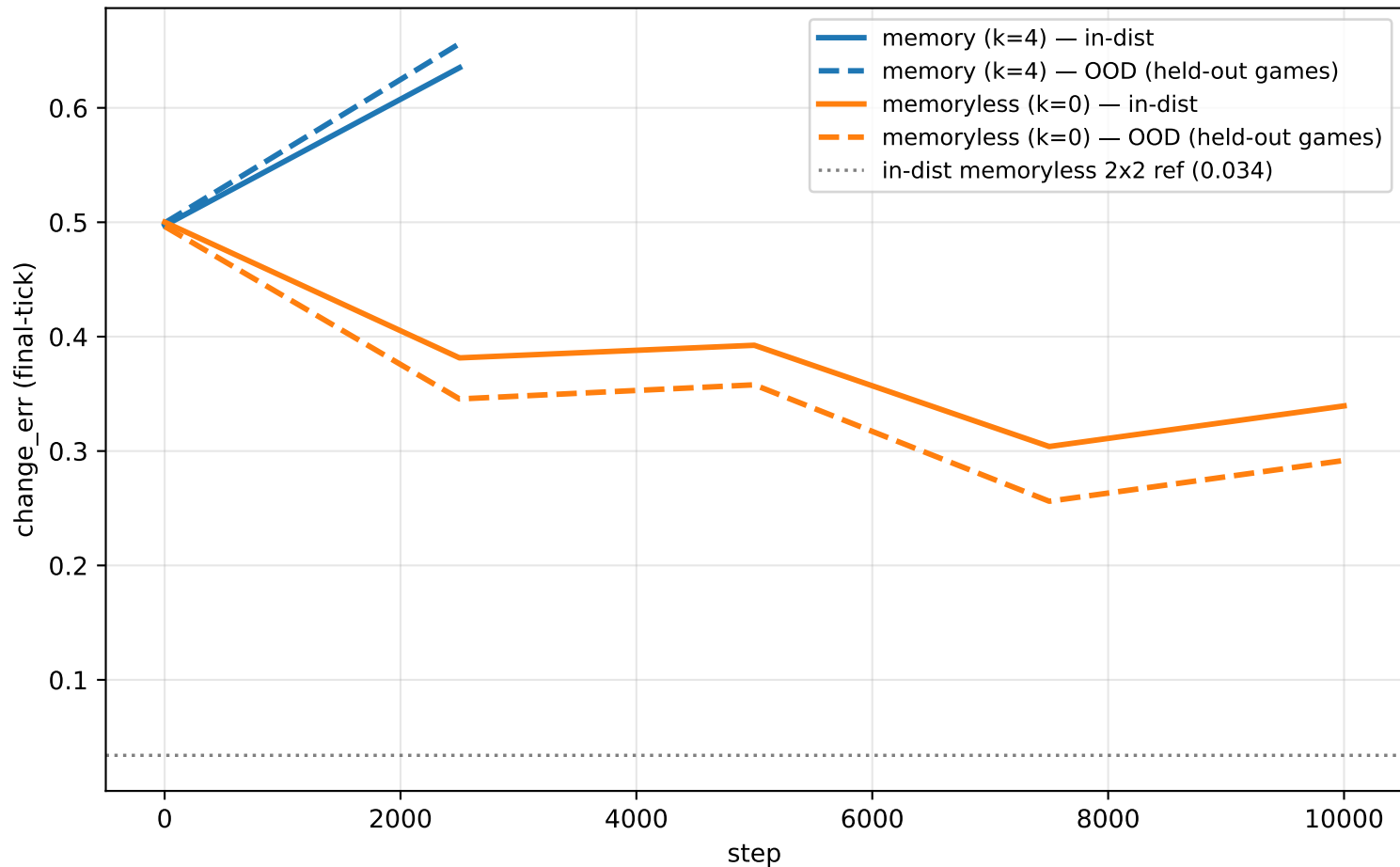
Recurrent memory vs memoryless: in-dist & OOD (800-game corpus, 708 train / 79 held-out games)
