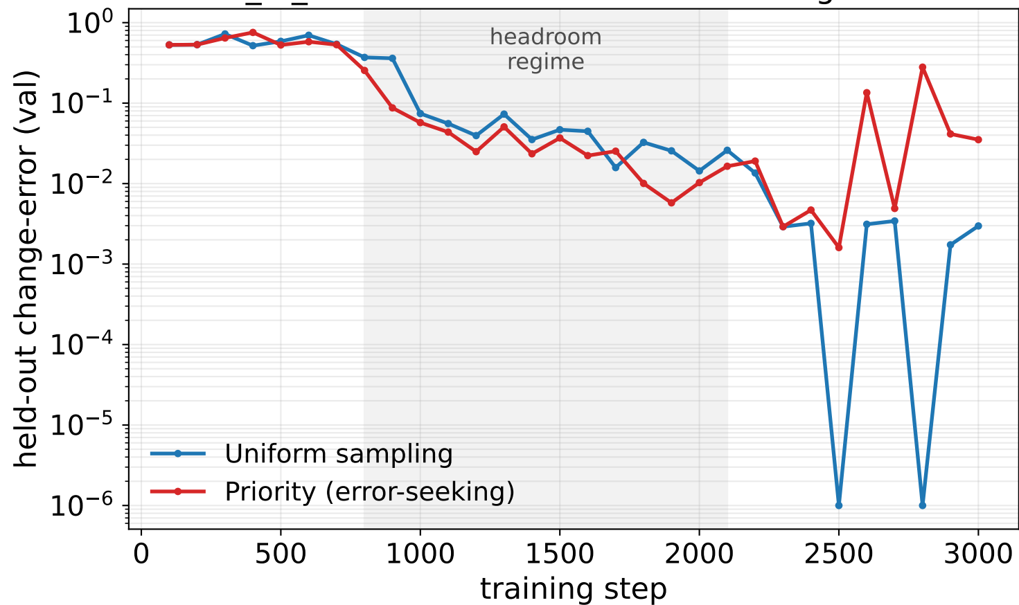
Heroes_of_Sokoban level 5 — error-seeking vs uniform
