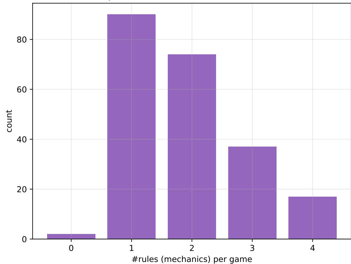
Final pool (220 envs): mechanics distribution
