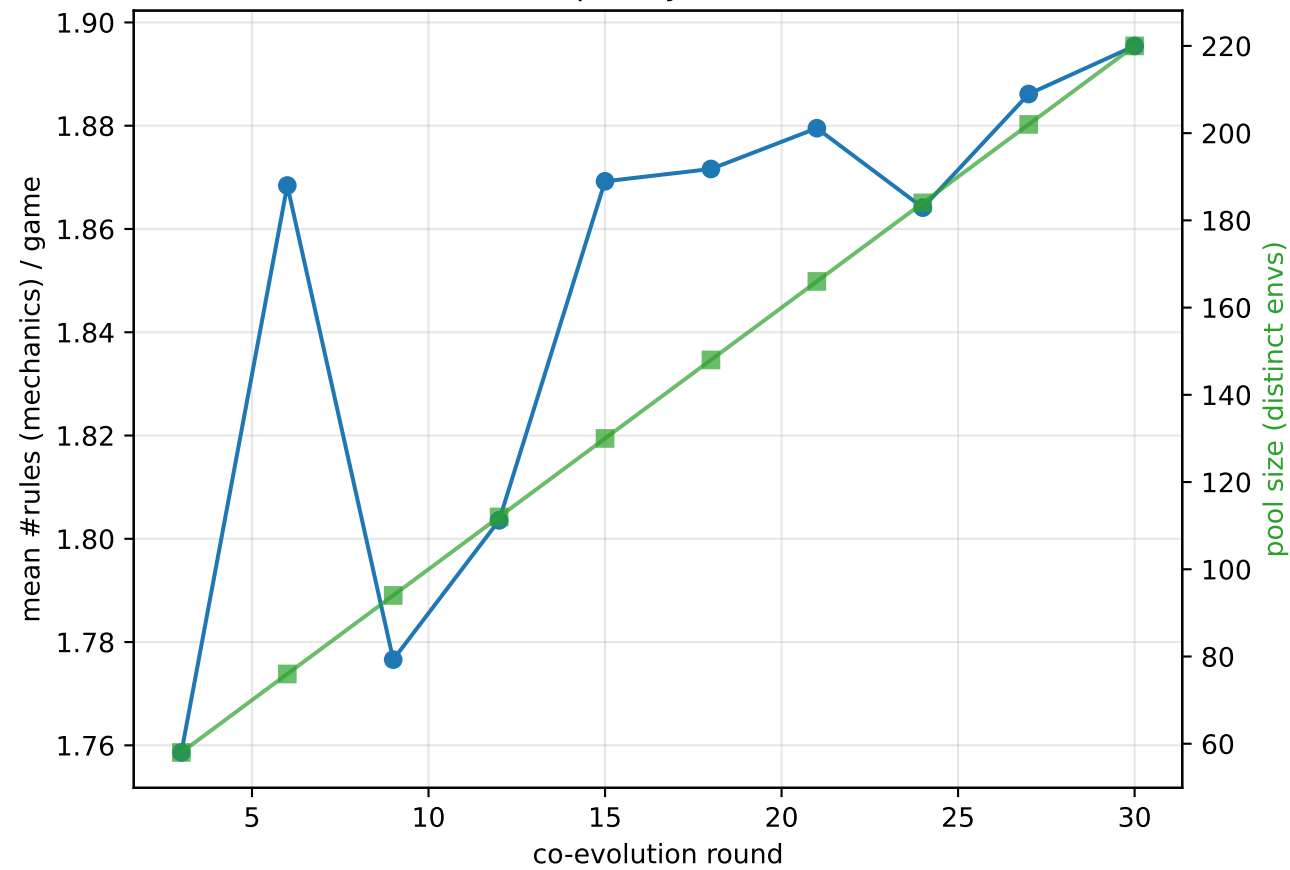
Pool complexity over rounds
