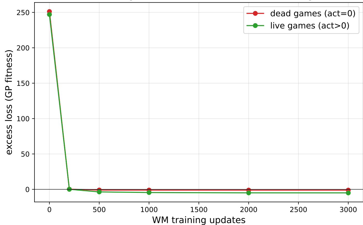
WM learns live games -> their fitness falls below dead games
