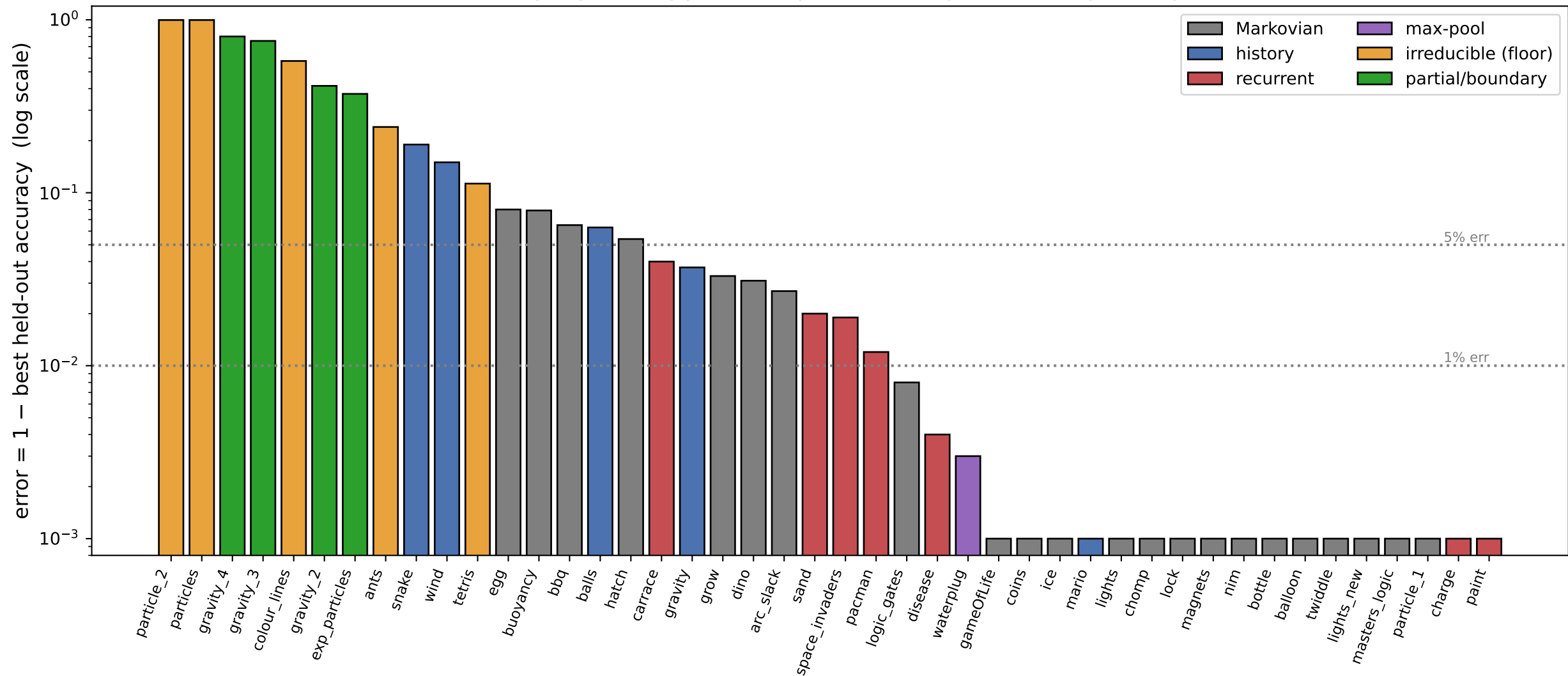
AutumnBench WM error per game (log y). Green=partial (active perfection loop); orange=irreducible floor.
