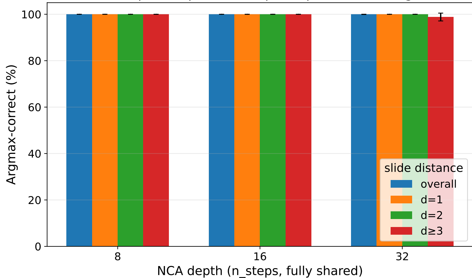
Varislide post-bitpack-fix: depth \times per-distance argmax
