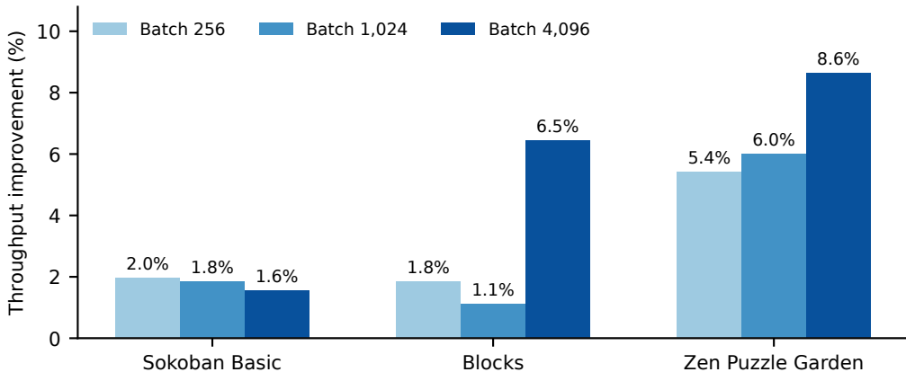
Movement-coordinate compaction · H200 · 15 paired trials
