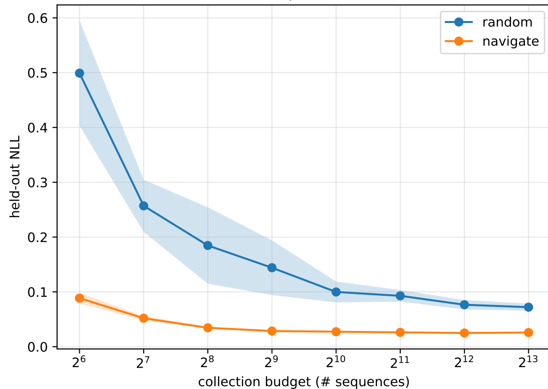
Full-sequence loss
