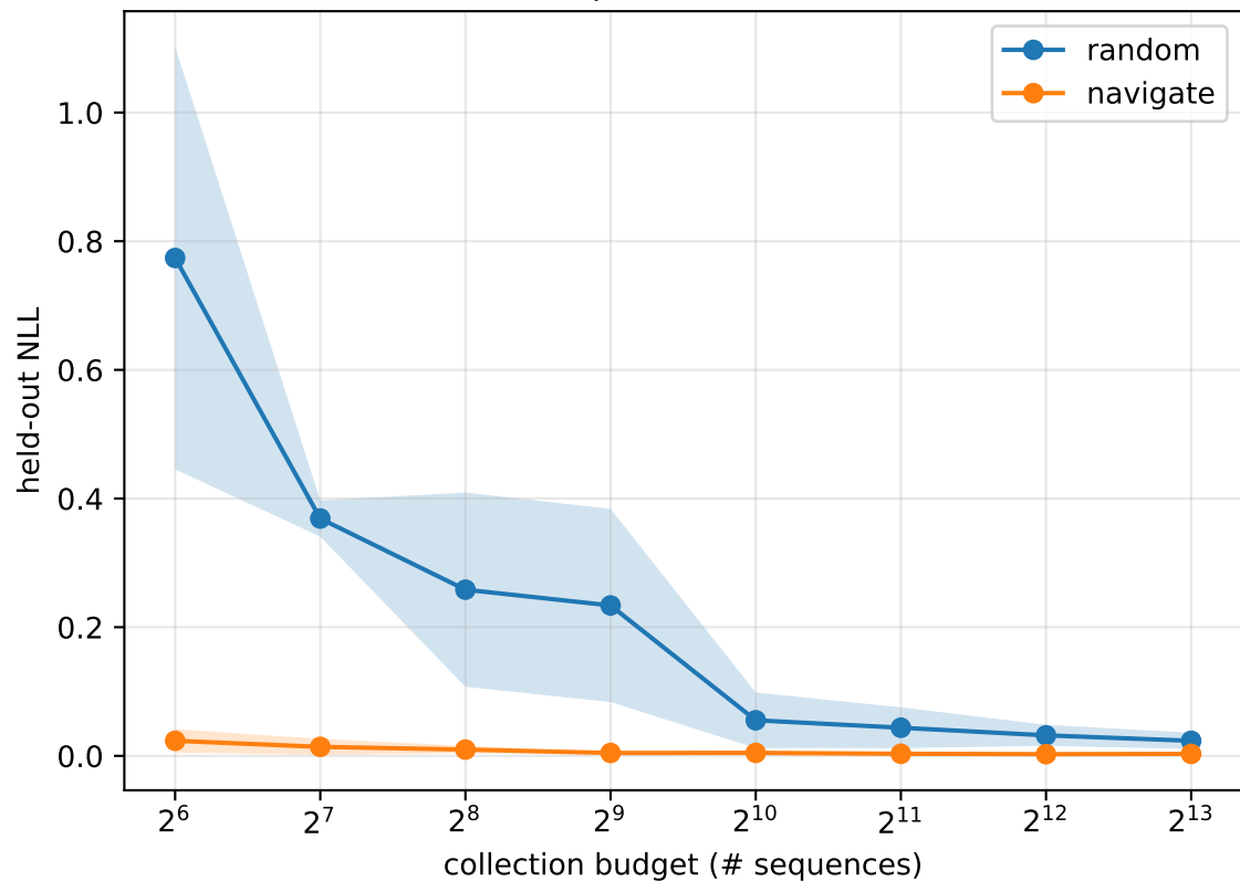
Resample-outcome loss
