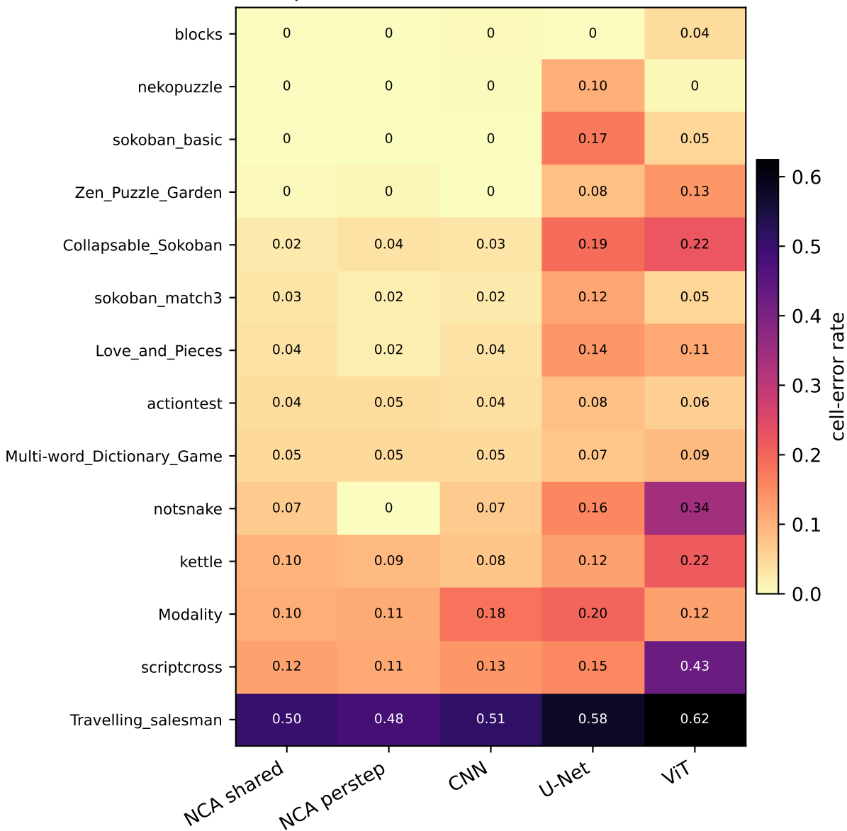
BFS final-step cell-error rate (mean over levels, then seeds)
