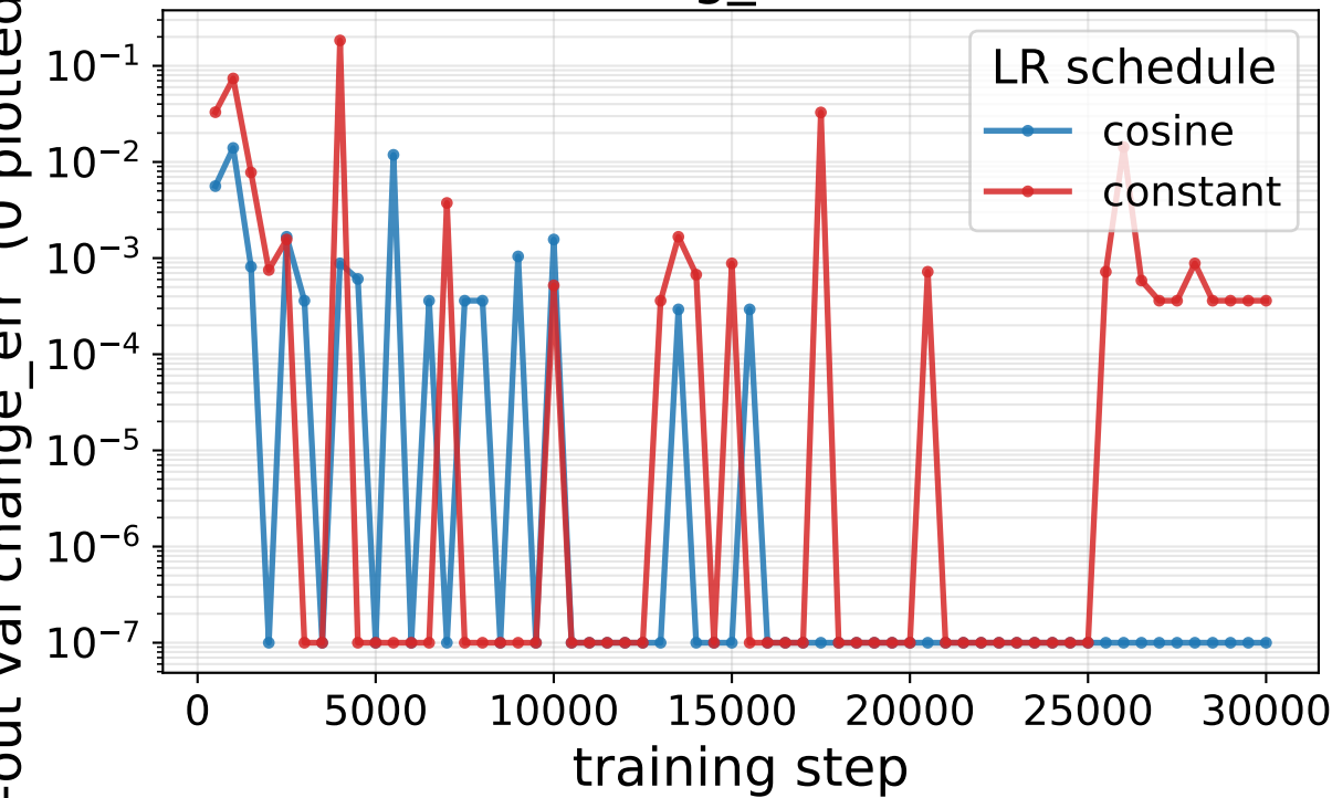
Travelling_salesman
