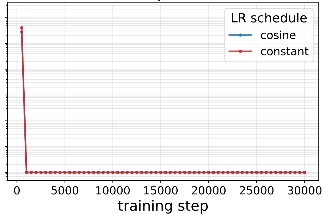
nekopuzzle
