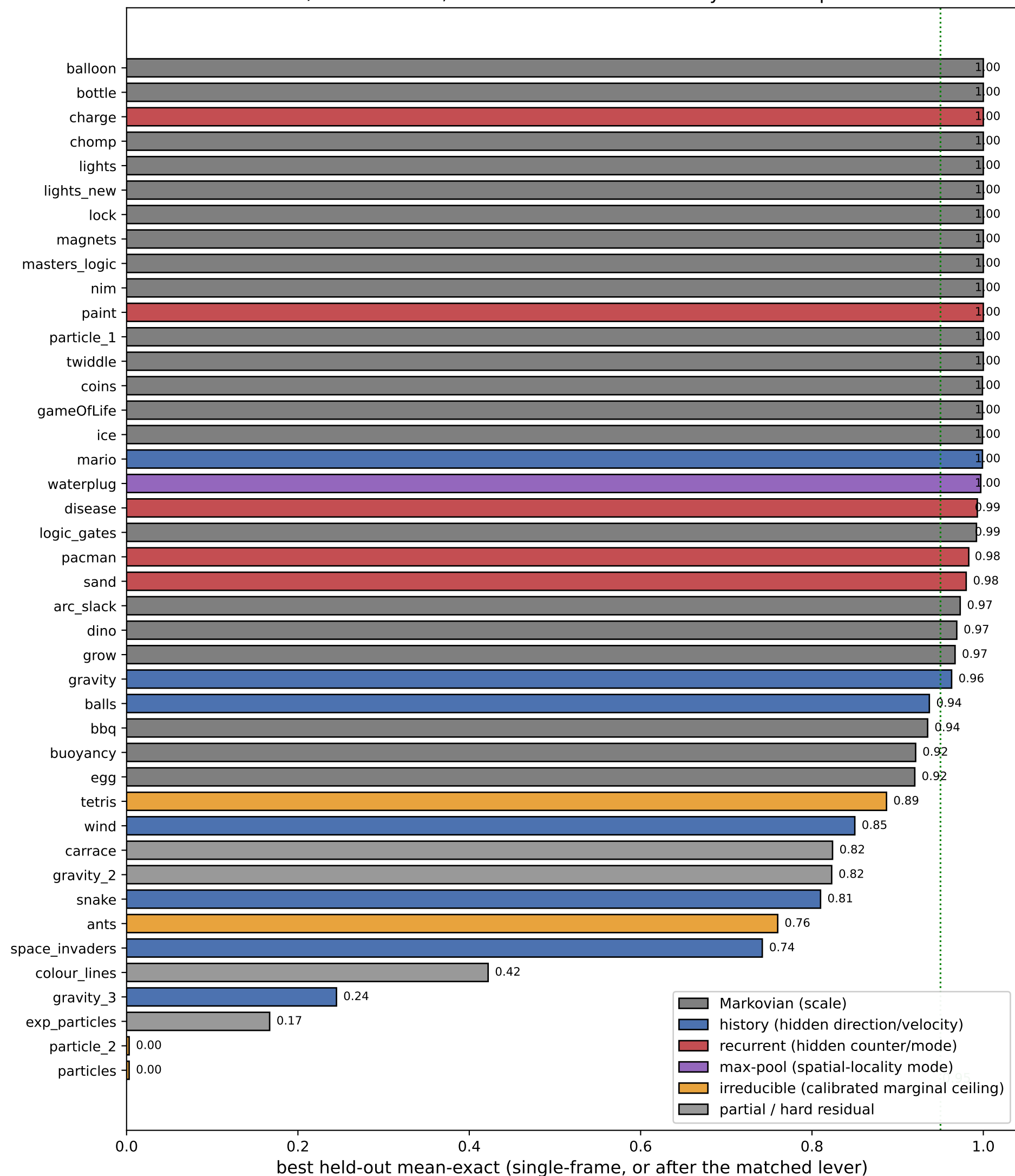
AutumnBench WM coverage: 42 environments by hidden-state class 26/42 at \geq 0.95 ; each color = the lever its dynamics require
