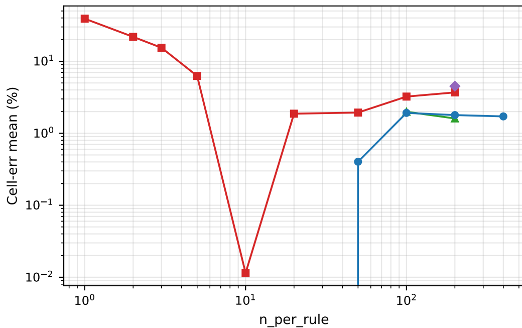
BFS solver
