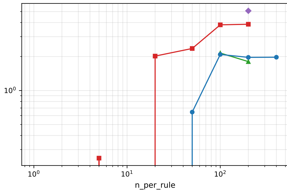
A* solver
