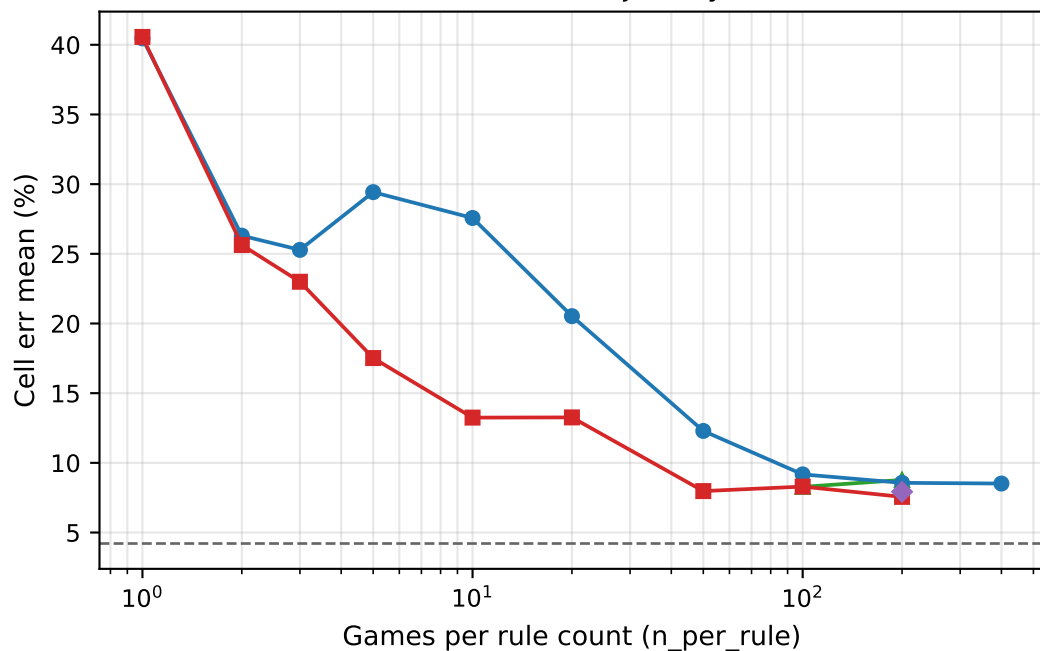
BFS solver trajectory
