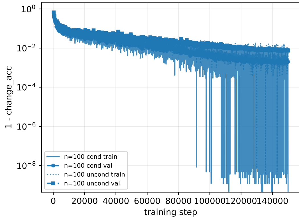
Train vs val (held-out 10%)
