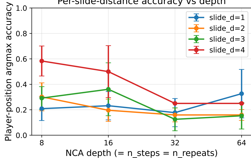
Per-slide-distance accuracy vs depth
