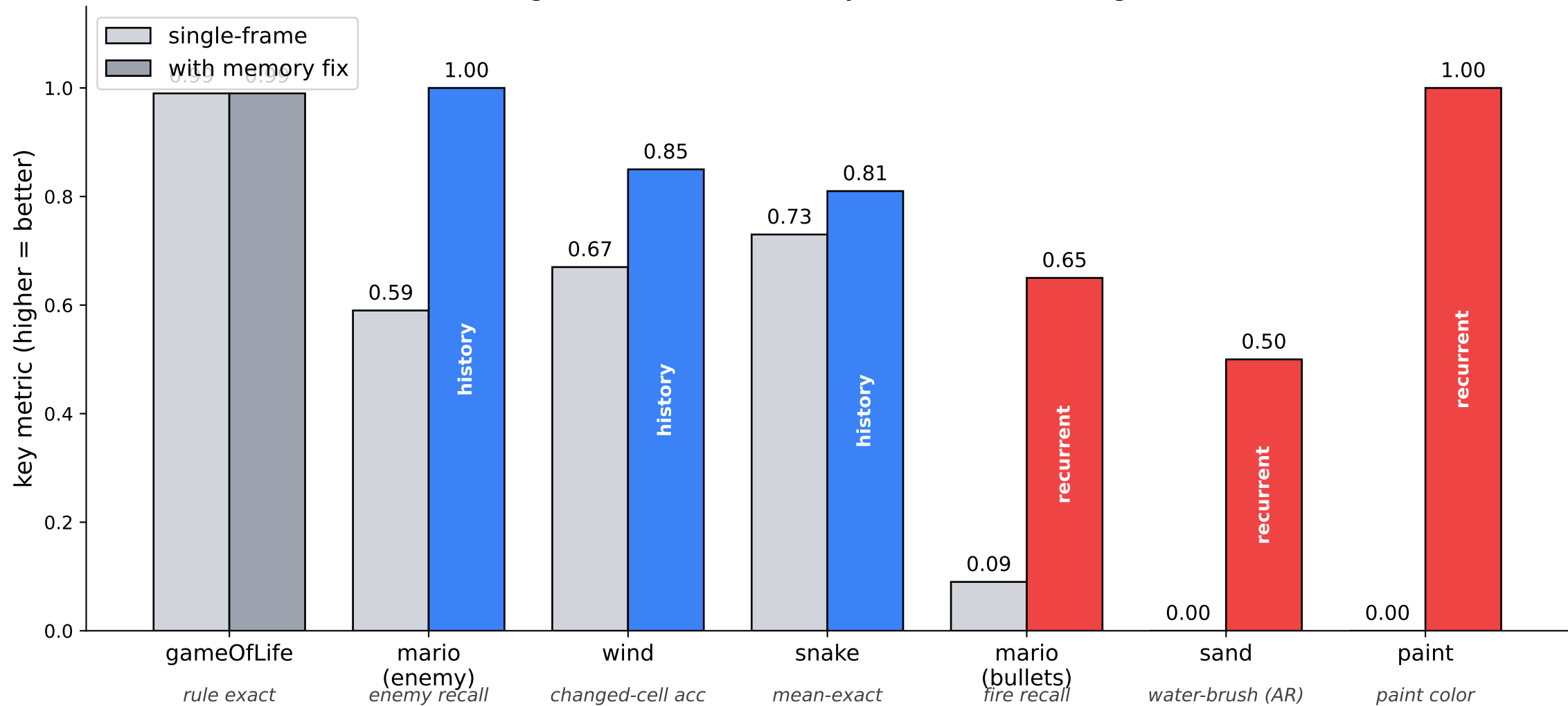
AutumnBench hidden-state blindspots and the memory fix (single-frame NCA vs. history / recurrent-hidden-grid)
