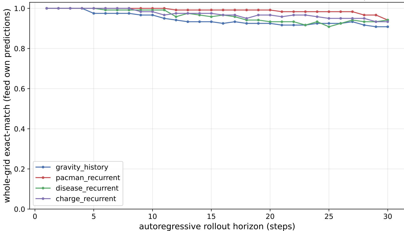
AutumnBench WMs are rollout-stable: exact-match holds over 30 AR steps
