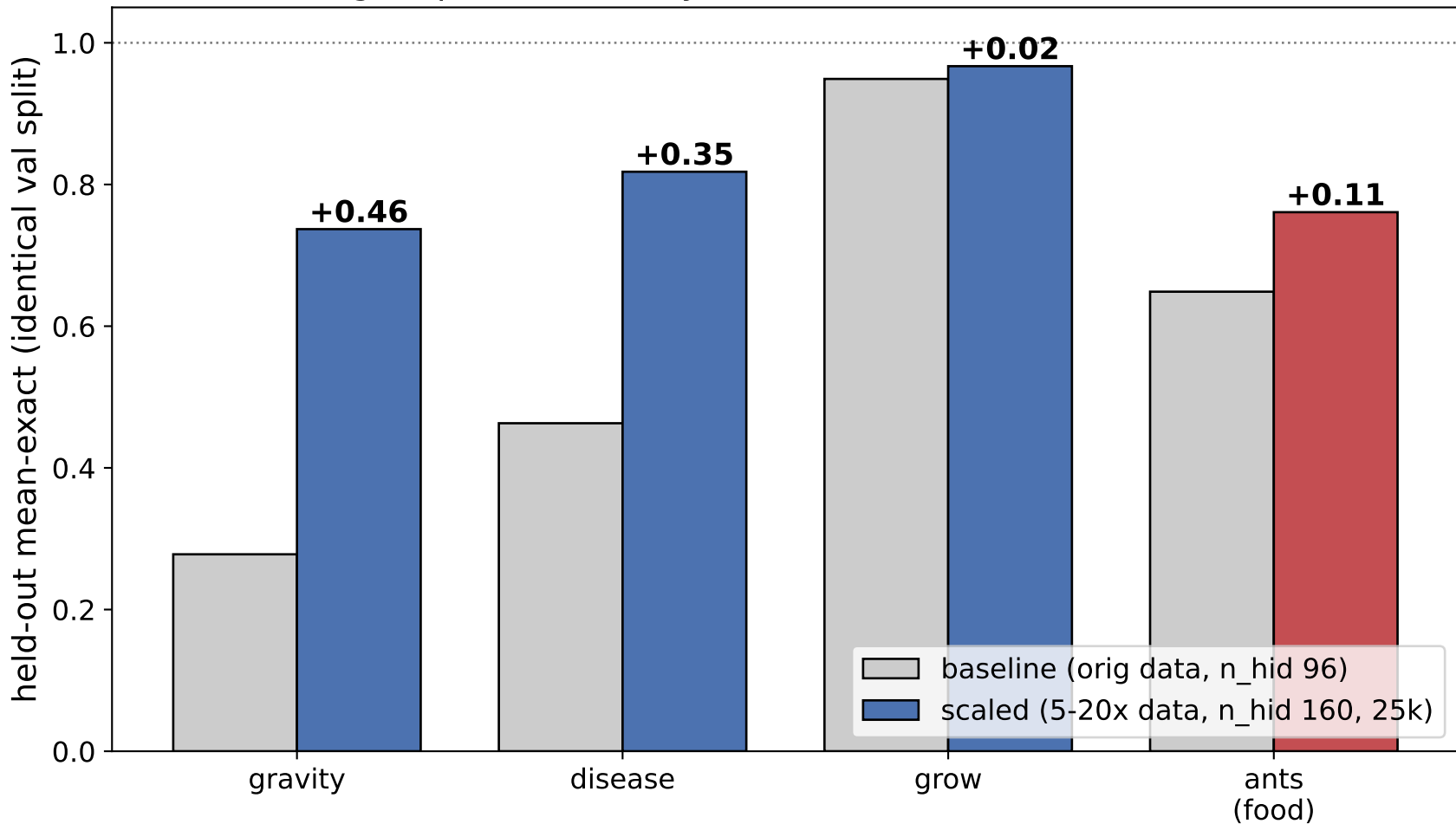
Scaling helps reducible dynamics, not irreducible randomness
