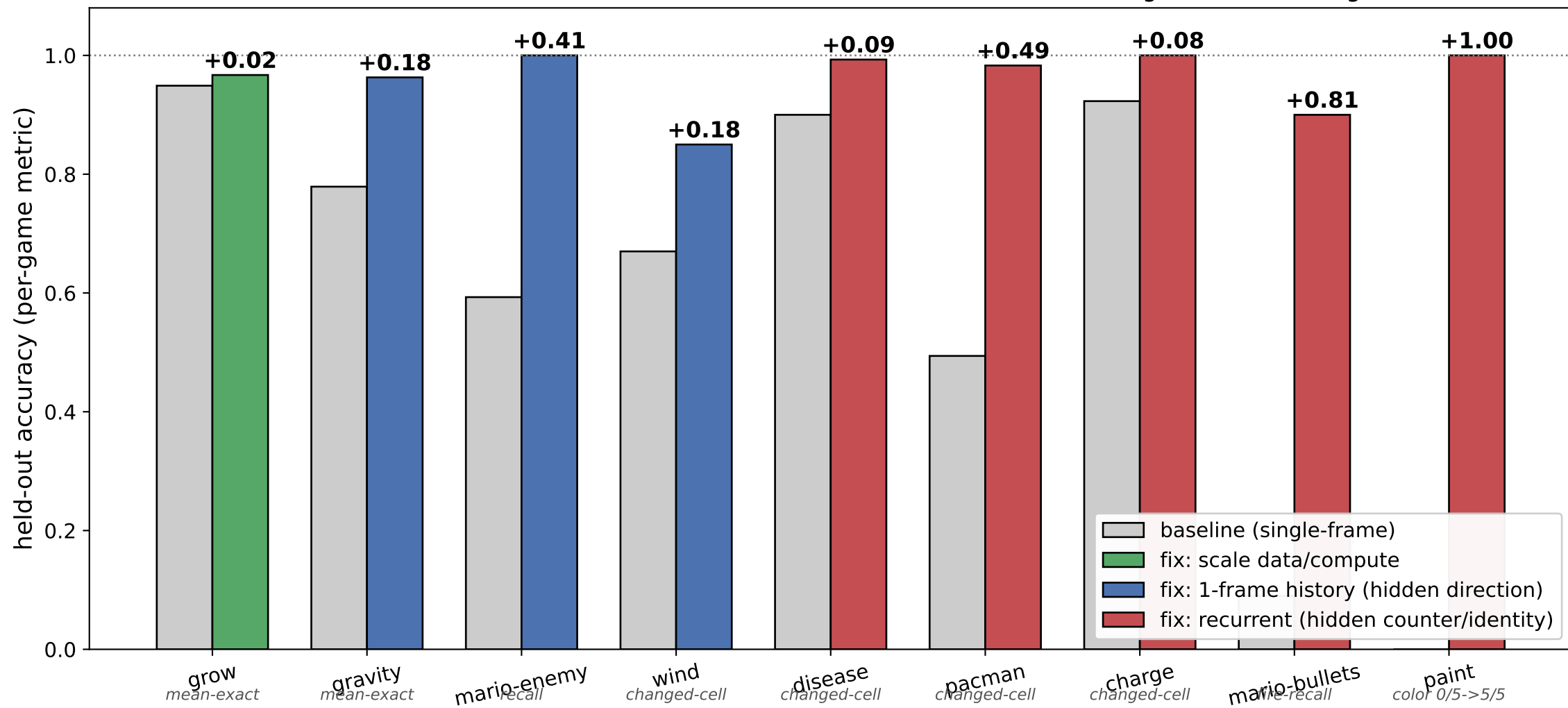
AutumnBench WM: each hidden-state class needs a distinct lever (ants food = 4th class: irreducible PRNG randomness → calibrated marginal is the ceiling)
