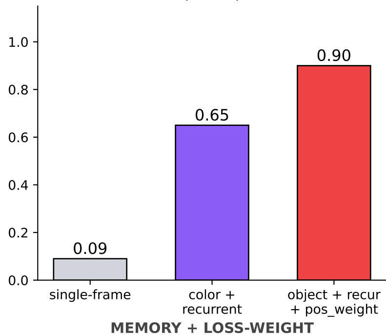
Bullet firing (recall)
