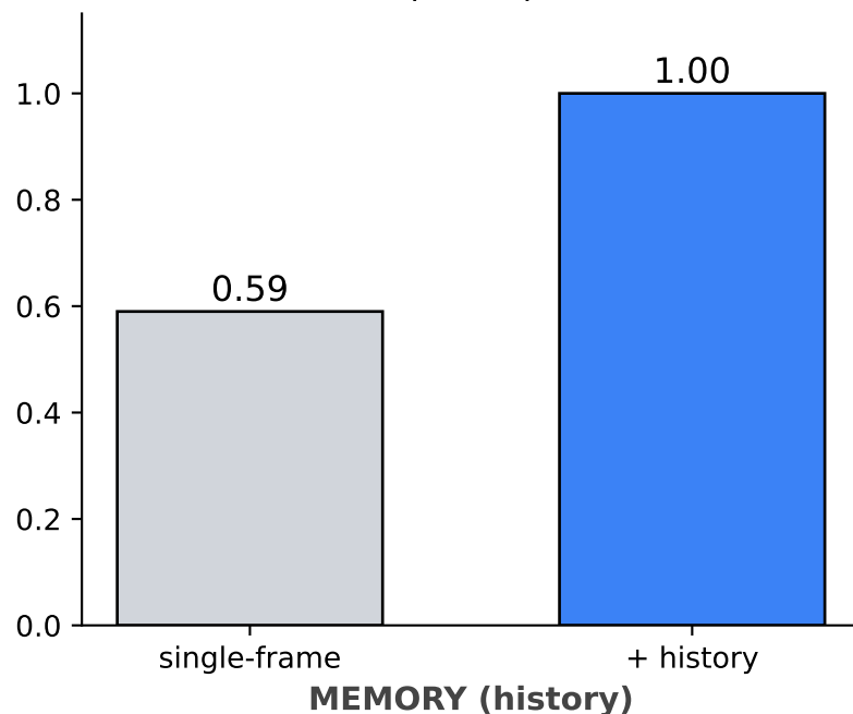
Enemy direction (recall)
