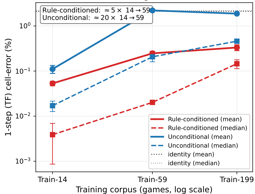
In-distribution (14-game intersection)
