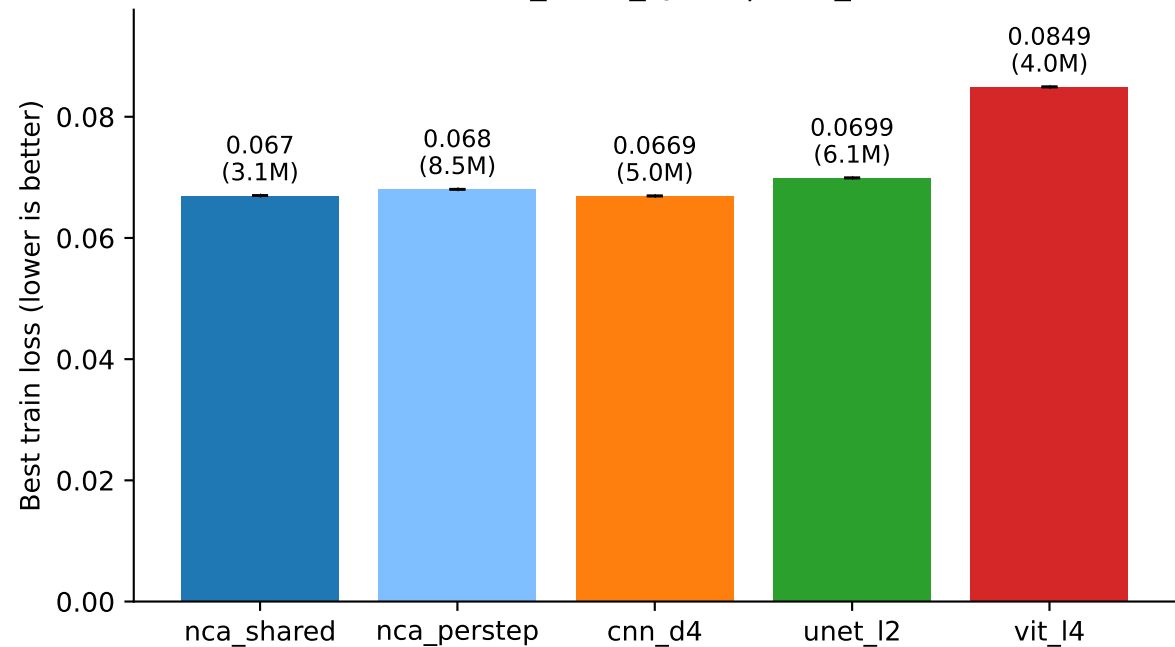
sokoban_basic_synth | best_loss
