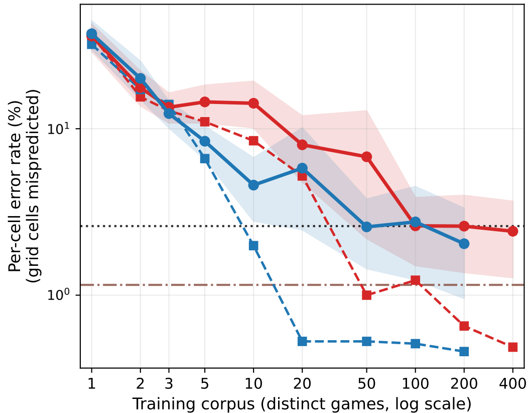
Out-of-distribution (Heldout-26)
