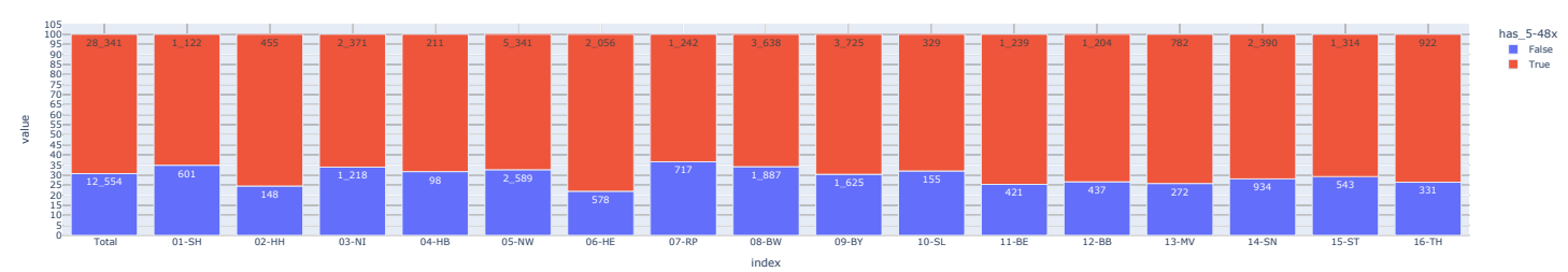
[z_kkr_label] by [has_5-48x], n=34 (40_895)
