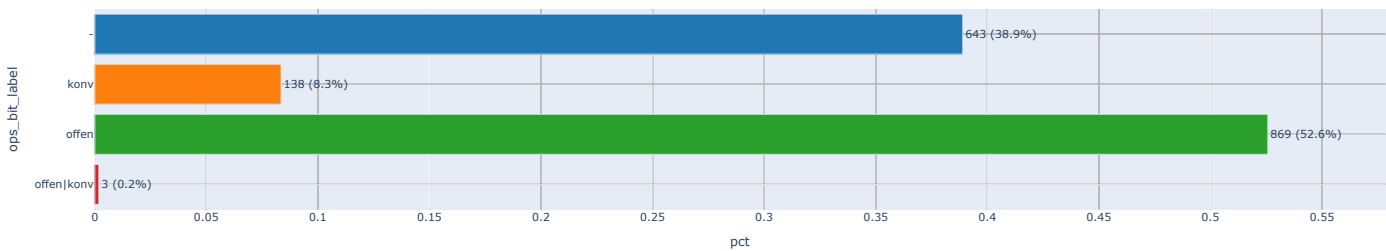
#5-422.2, [count] by [ops_bit_label], n=4 (1_653)
