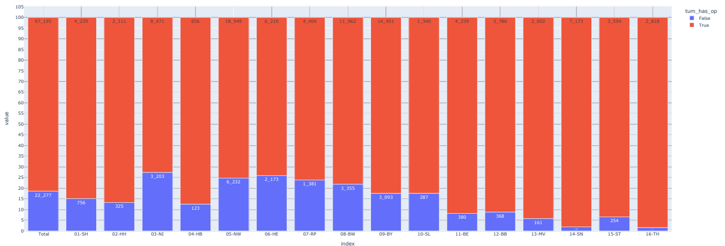
#c18_t(p)=1-4, [z_kkr_label] by [tum_has_op], n=34 (119_472)
