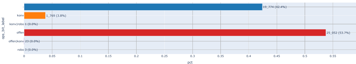
#5-422.4, [count] by [ops_bit_label], n=6 (46_622)
