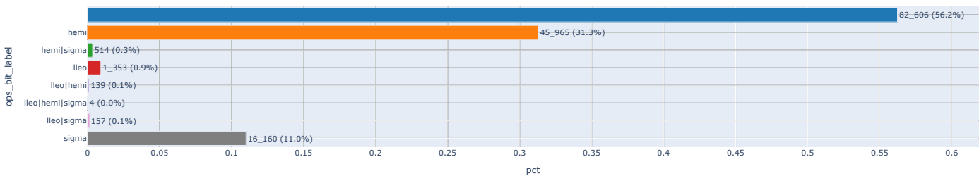
#5-422, [count] by [ops_bit_label], n=8 (146_898)
