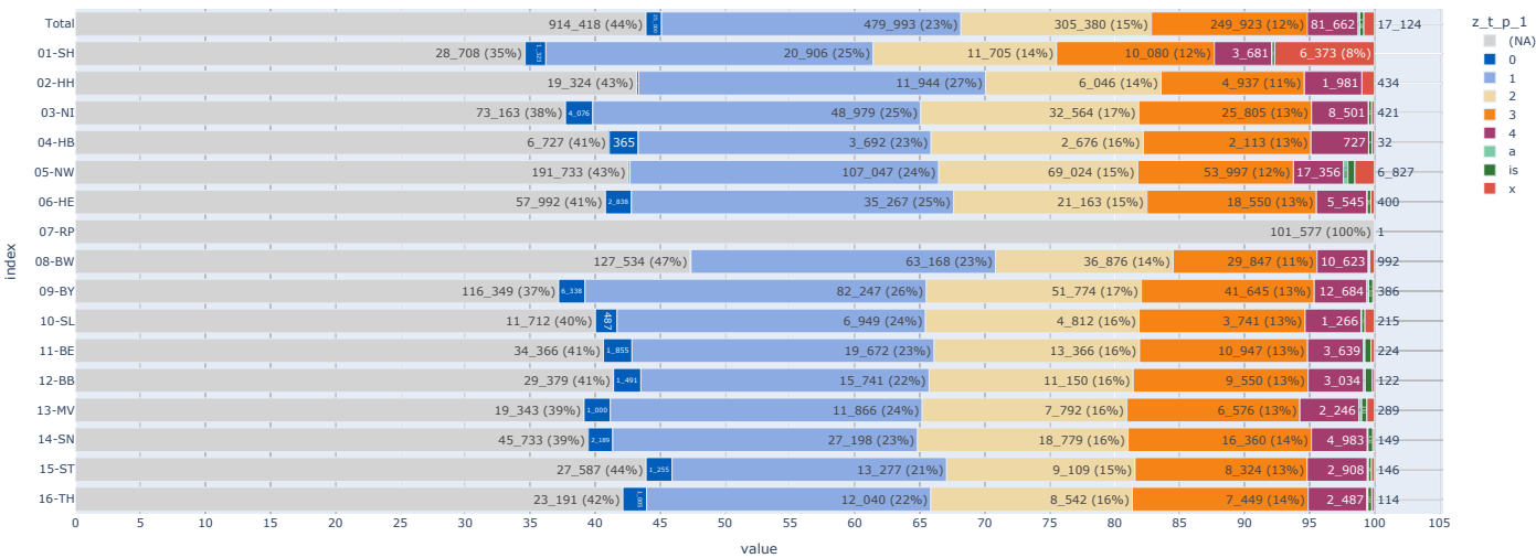
[kk] by [z_t_p_1], n=2_082_538
