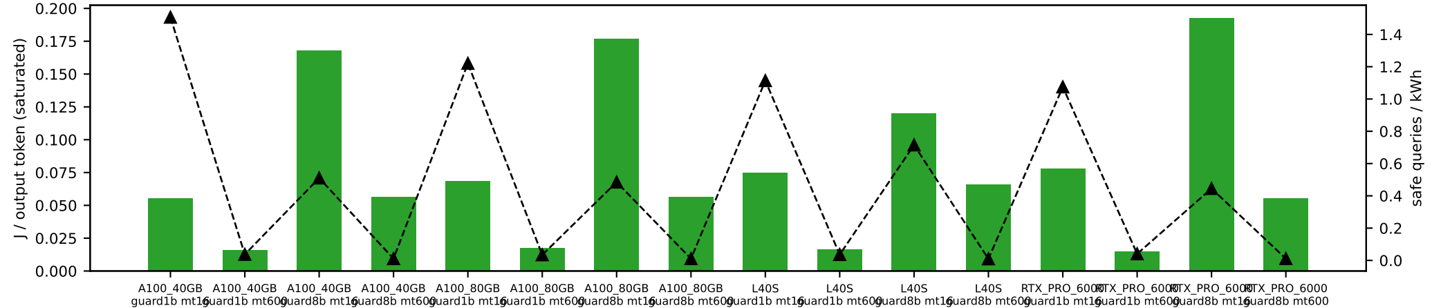
Energy cost of safety checks by hardware and mechanism
