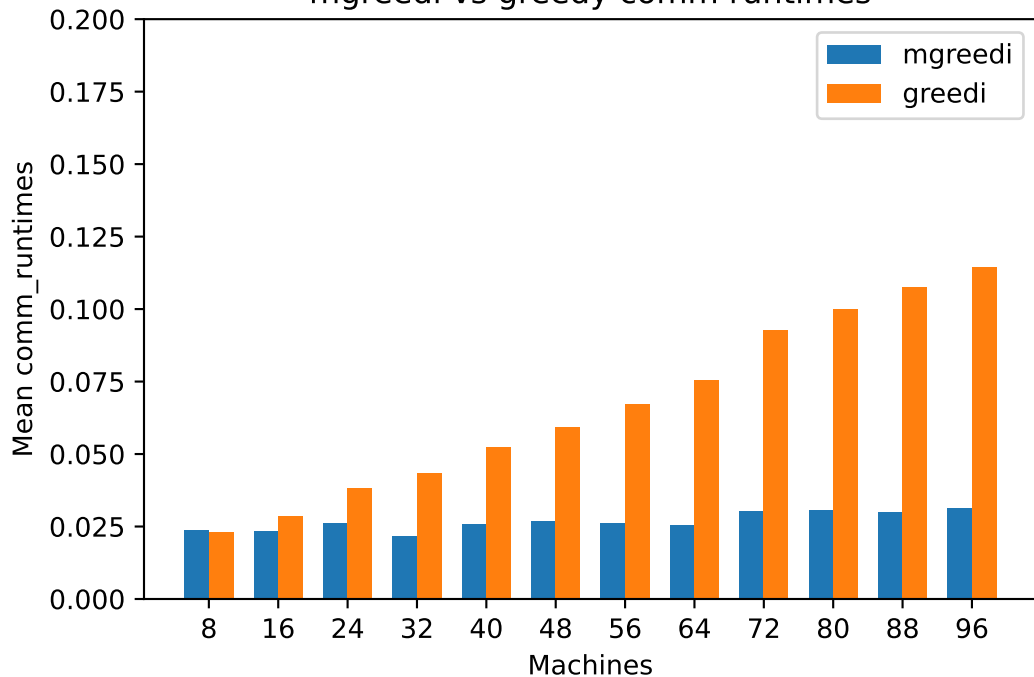
mgreedi vs greedy comm runtimes
